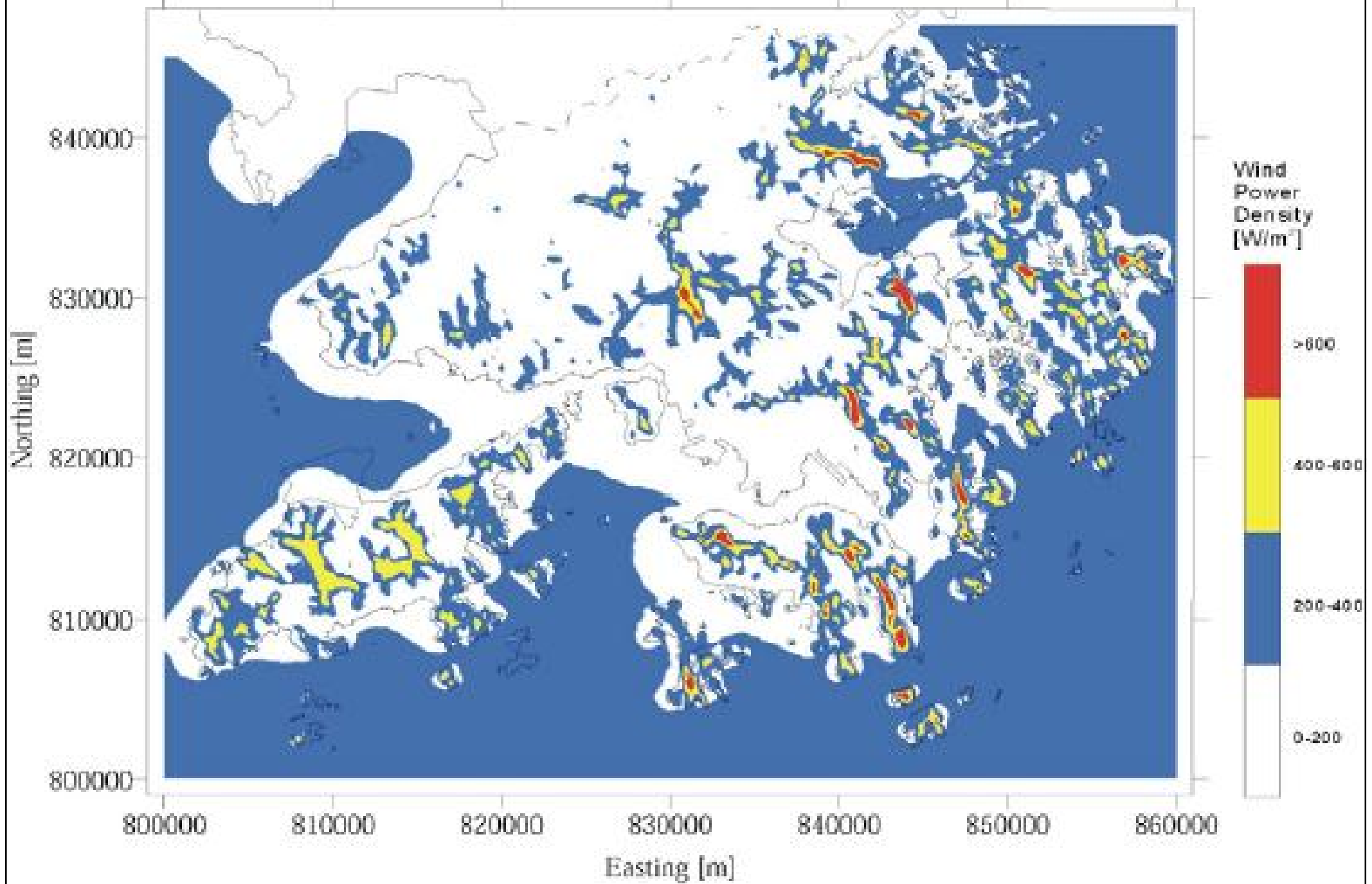
Wind power density over the region of Hong Kong (from EMSD)
