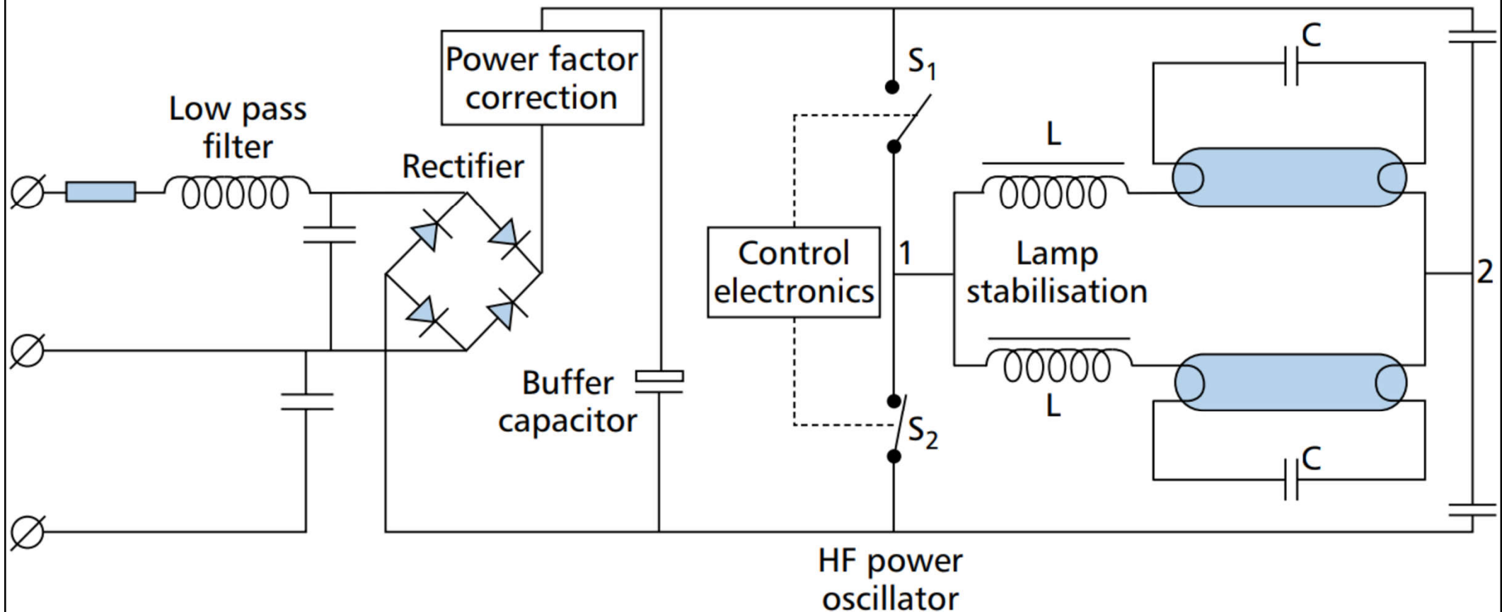
Wiring Diagram
