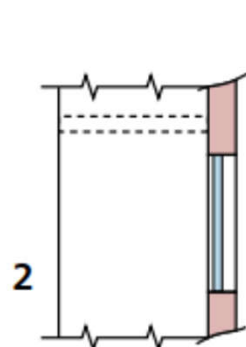
Fixed vertical projection
