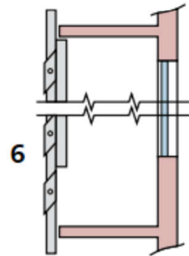
Pivoted non-retractable louvre
