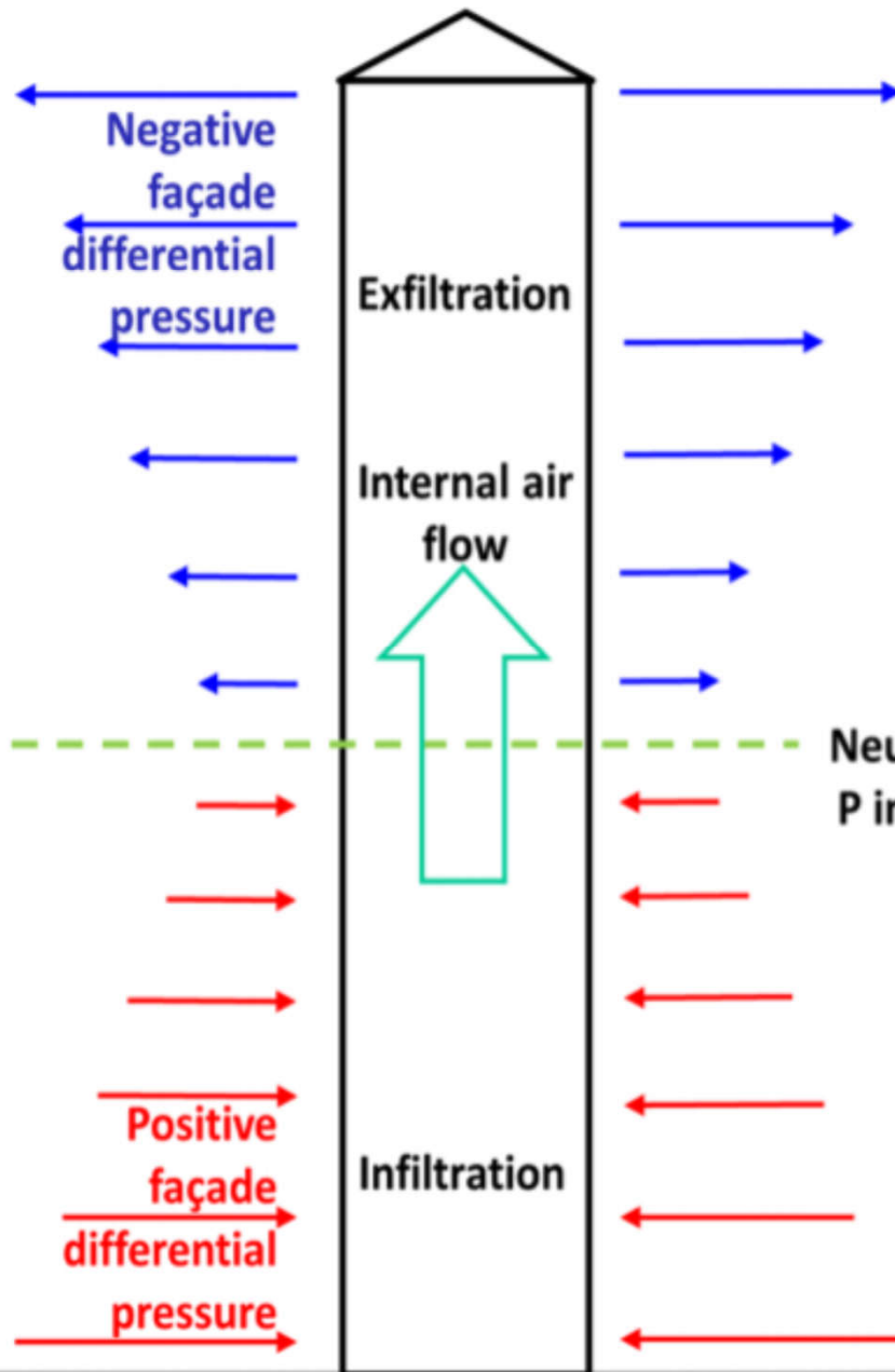
a) Stack effect
