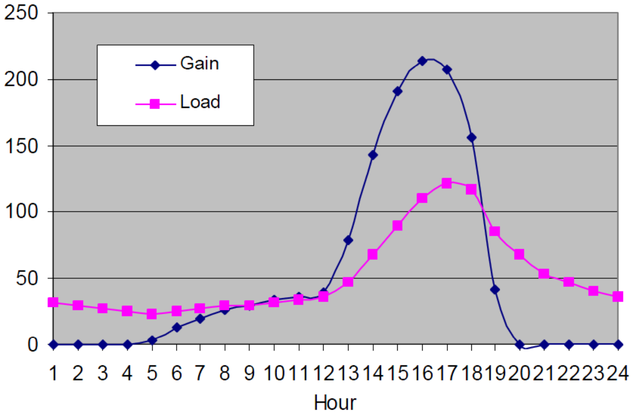
Solar cooling load vs. heat gain (July, west) (latitude 48 deg N)
