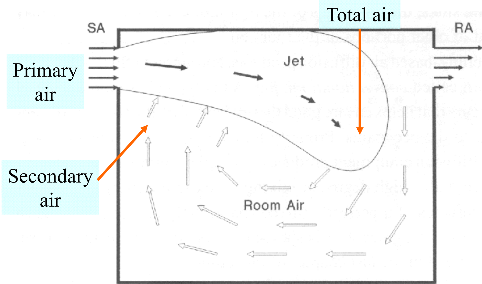
"Entrainment" or "Conventional-Mixing" Flow
