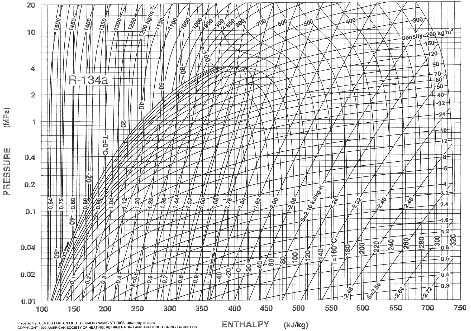
Pressure-Enthalpy Diagram for Refrigerant 134a
