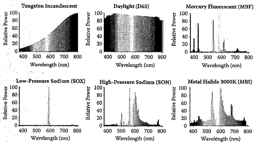
FIGURE E.1 Emission spectra of various lamps.
