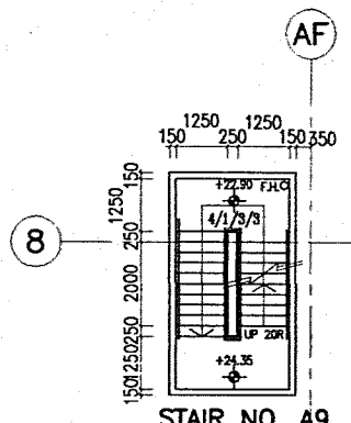
STAIR NO. A9 PART PLAN AT LEVEL +24.35
