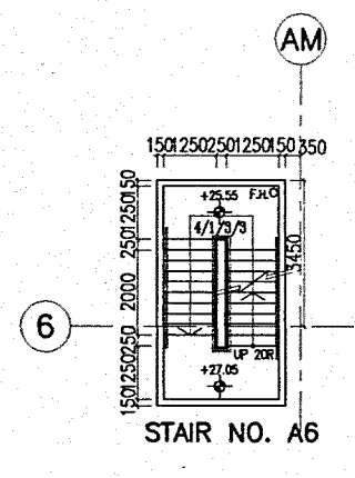
STAIR NO. A6 PART PLAN AT LEVEL +27.05
