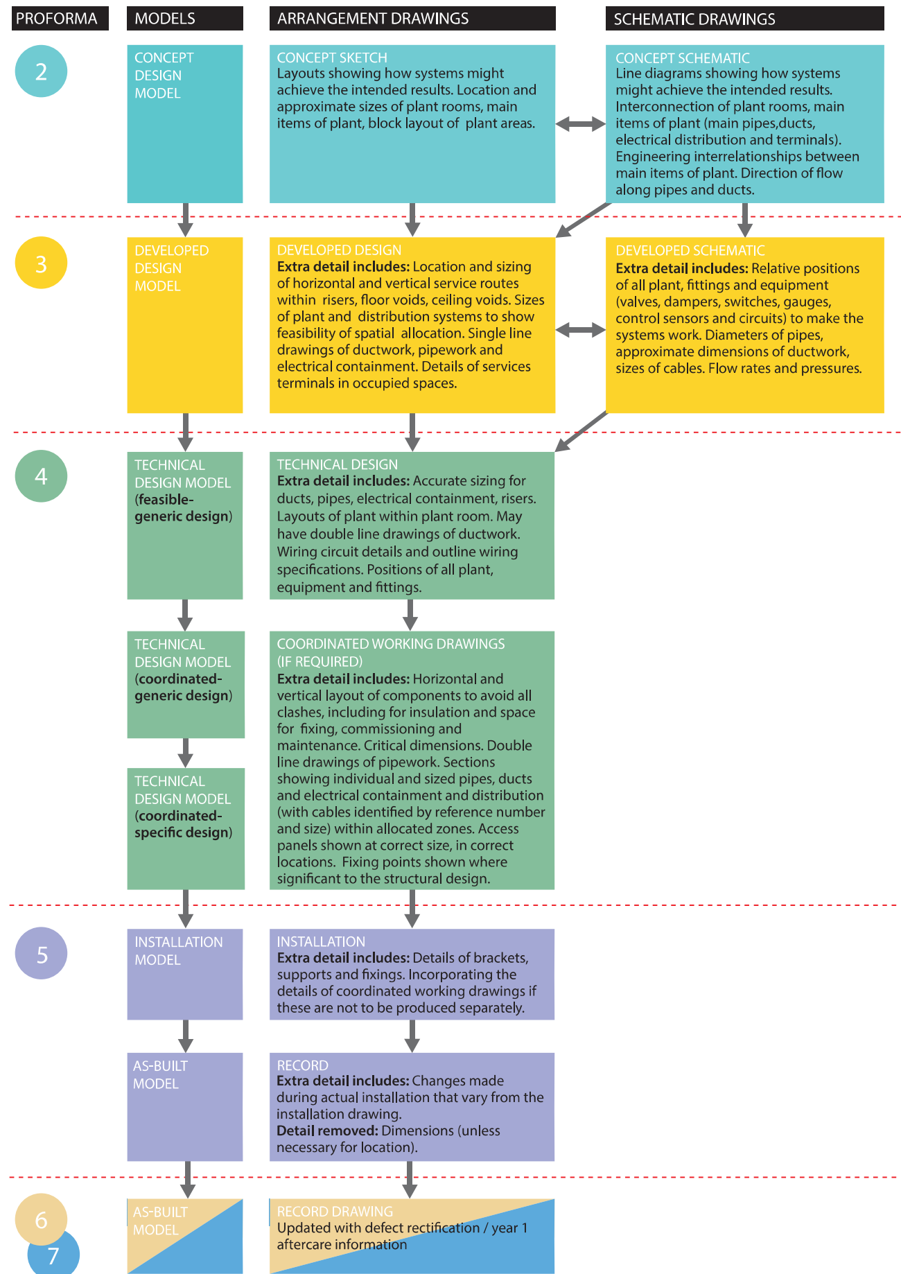
Figure 2: Design outputs flow chart
