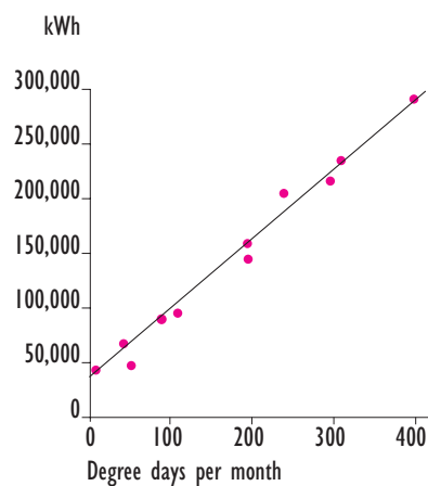
Example monthly heating energy use in a well controlled building
