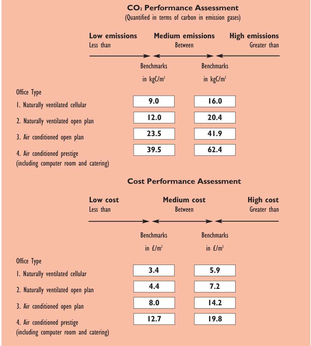
Figure A1.4 Carbon Dioxide Emission and Cost Benchmarks
