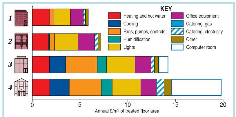
Figure 5.2: Typical energy cost breakdown
