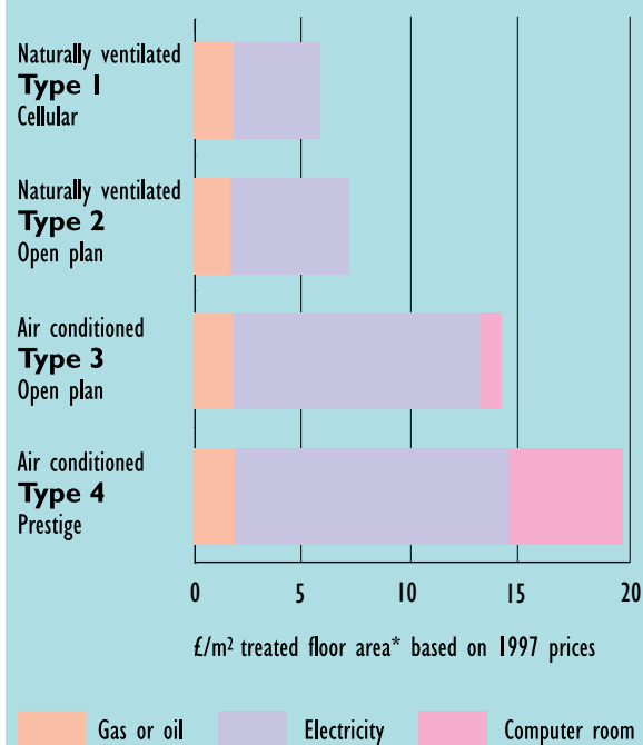
Figure 5.1 Typical Energy Costs of Office Buildings
