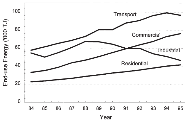
Fig. 6. Energy end-use in Hong Kong, 1984–95.
