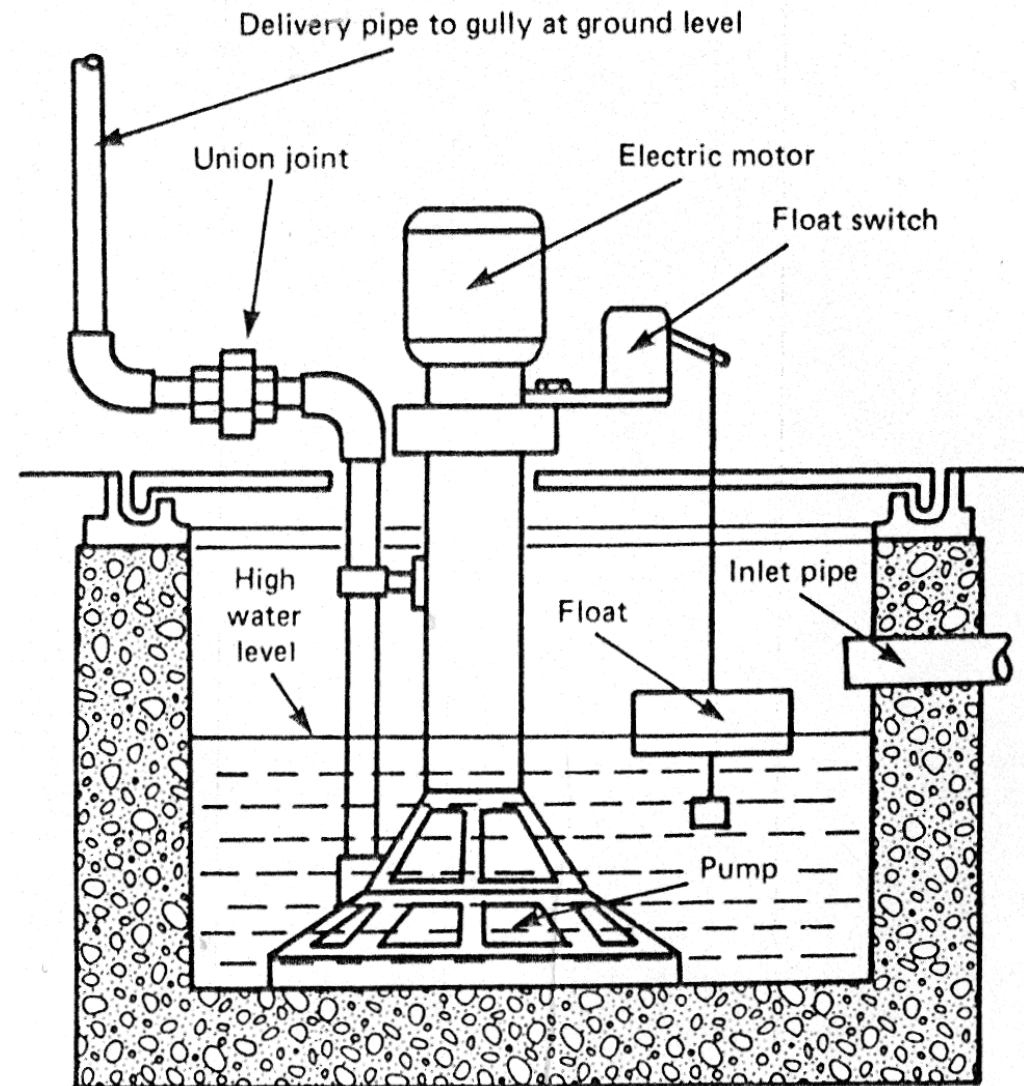
Sump pump
