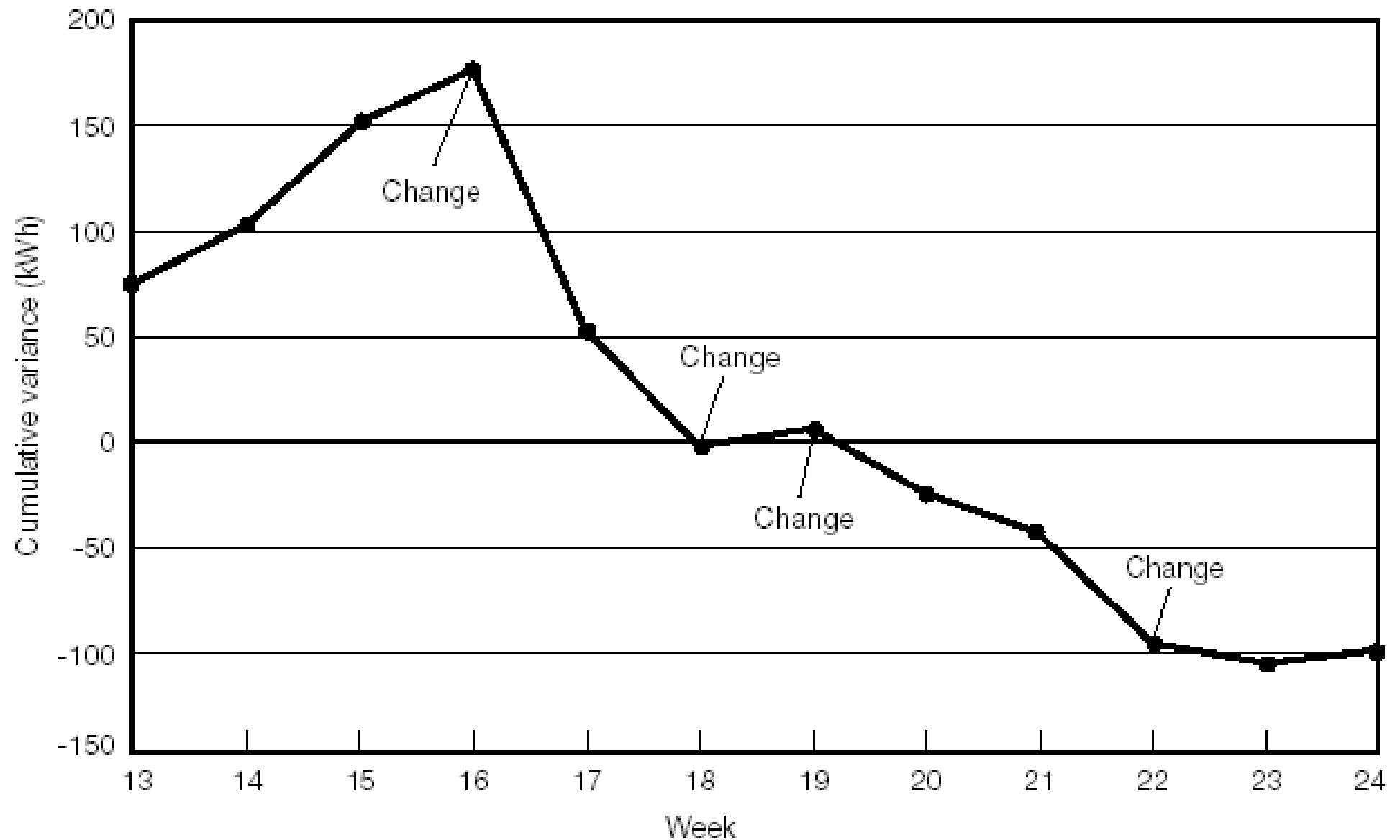
CUSUM chart
