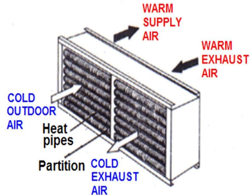
Heat pipe array intalled between two airstreams
