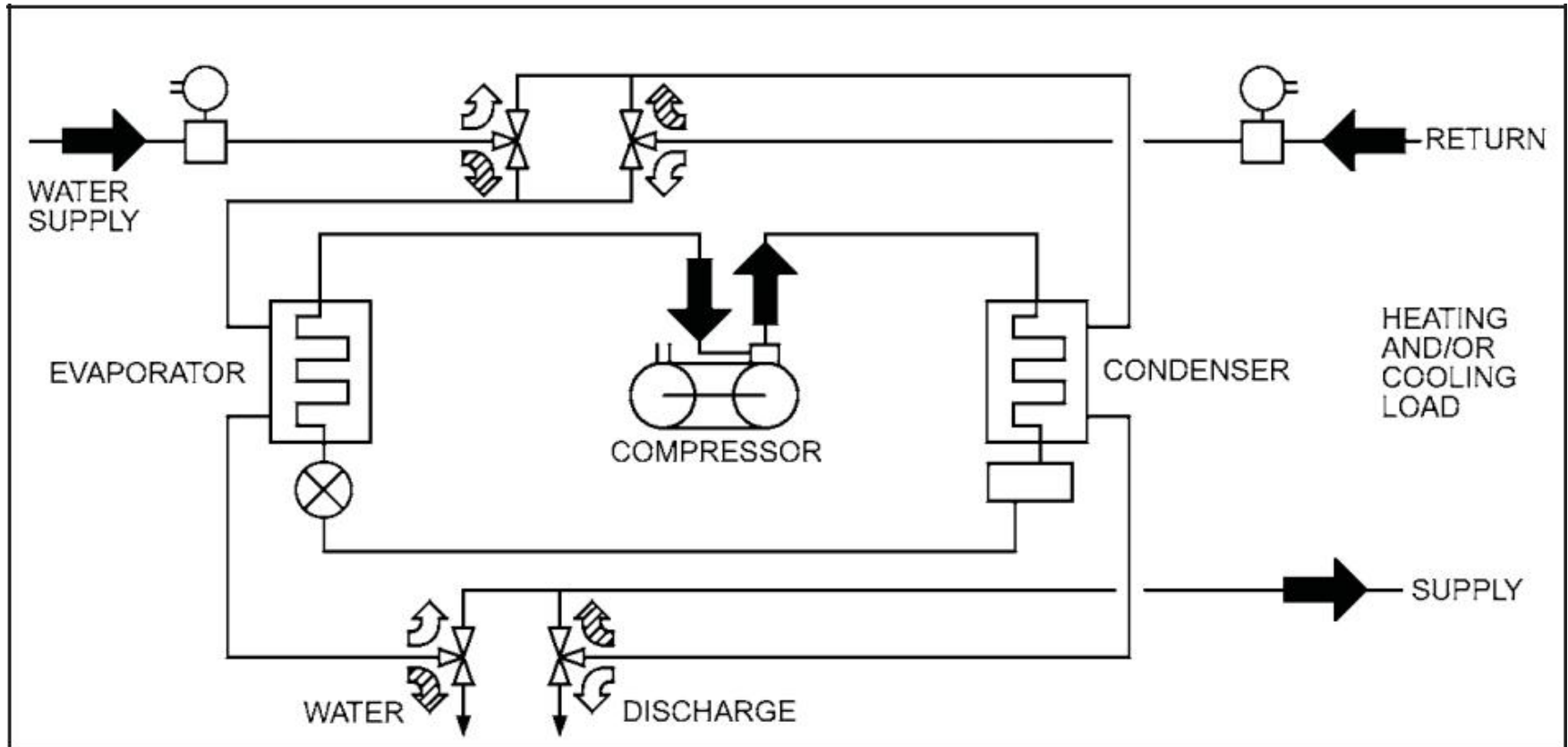
Water-to-water heat pump
