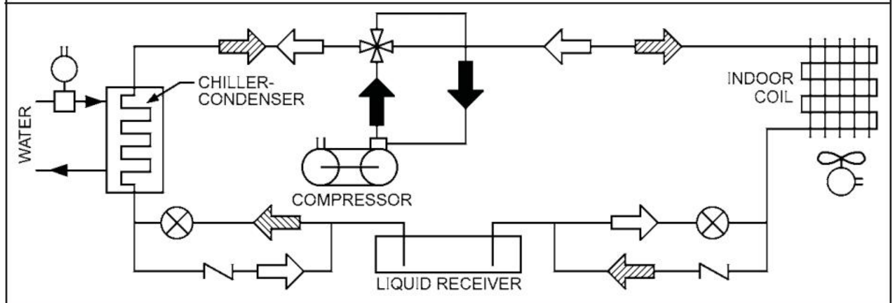
Water-to- air heat pump
