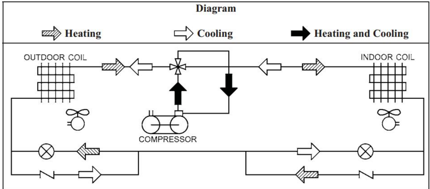
Air-to-air heat pump
